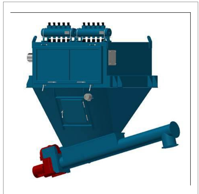
Powervac filter with conical bottom discharge and screw.
